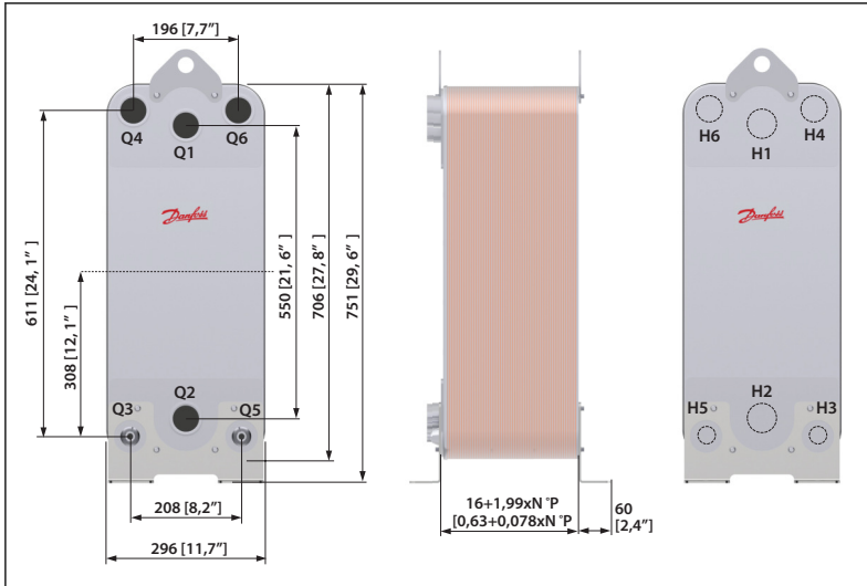
Figure 1: Dimensions
