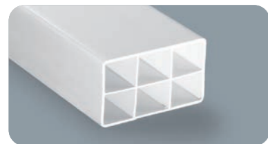
AC 70X40 Breaking resistance for meter 6217 Kg
