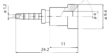
81900104 Inserto 180° Femmina a 3 Vie 180° Tee Female Nipple
