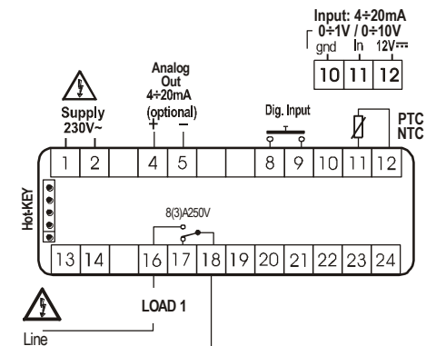
Probe: Pt100=11 - 10 (12); Thermocouple J, K, S= 11(+)- 10(-) 115Vac supply: 1-2; 24Vac supply: 1-2
