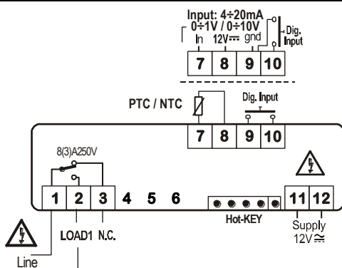
Probe: Pt100= 7 - 9 (8); Thermocouple J, K, S = 7(+); 9(-) 24Vac/cd supply: 11-12
