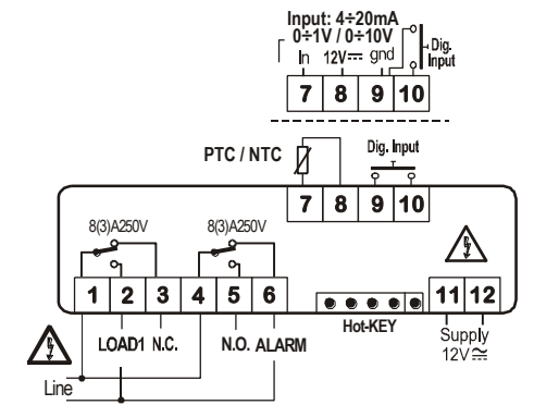
Probe: Pt100= 7 - 9 (8); Thermocouple J, K, S = 7(+); 9(-) 24Vac/cd supply: 11-12
